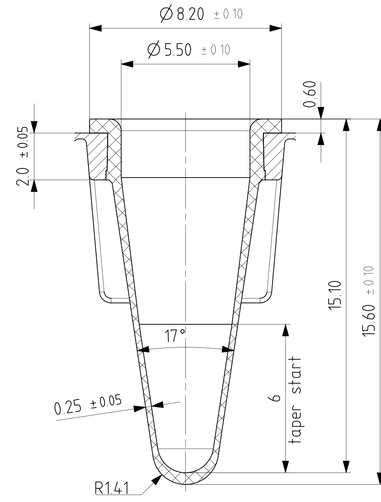
VIAL FORM 96 pos SCALE 10:1
