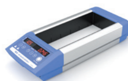
Dry Block Heater 3 Ident. No. 0004025300
